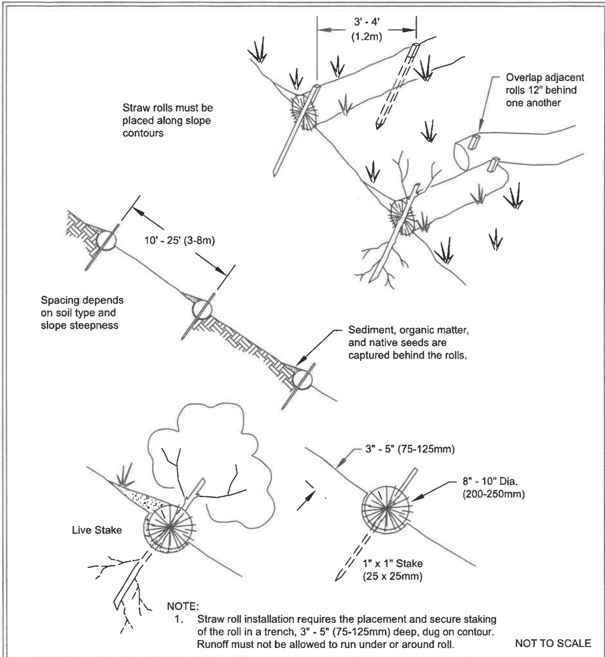
Figure II-4.24: Wattles
