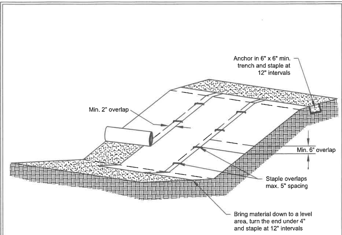
Figure II-4.4: Slope Installation
