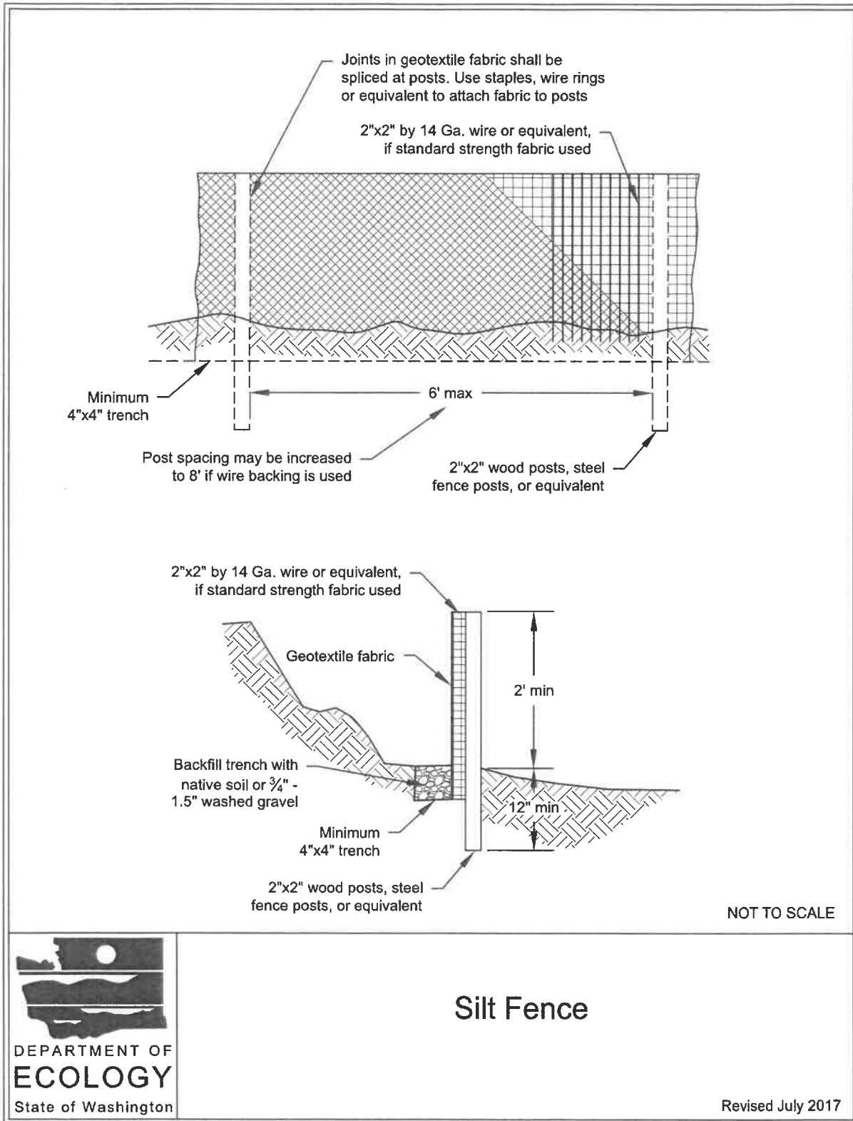
Figure II-4.22: Silt Fence
