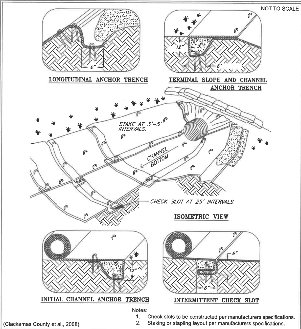
Figure II-4.3: Channel Installation
